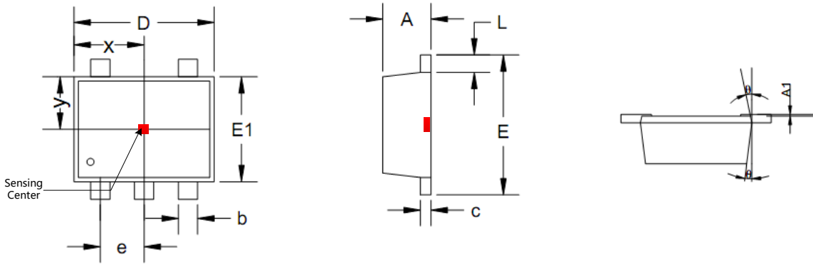
Figure.15 SOT-553 Package Drawing
