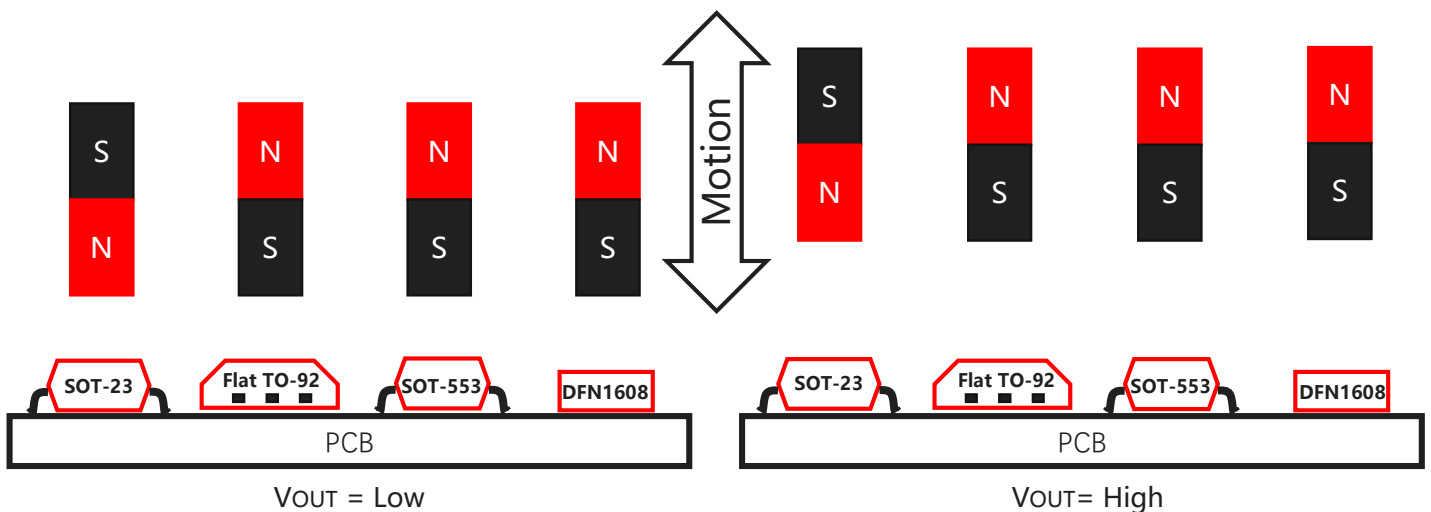
Figure.3 Flux Direction Polarity
