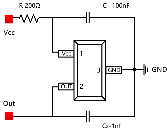
Figure.9 Harsh Environment Application Circuit Note: Min Supply Voltage \geq 2.0V
