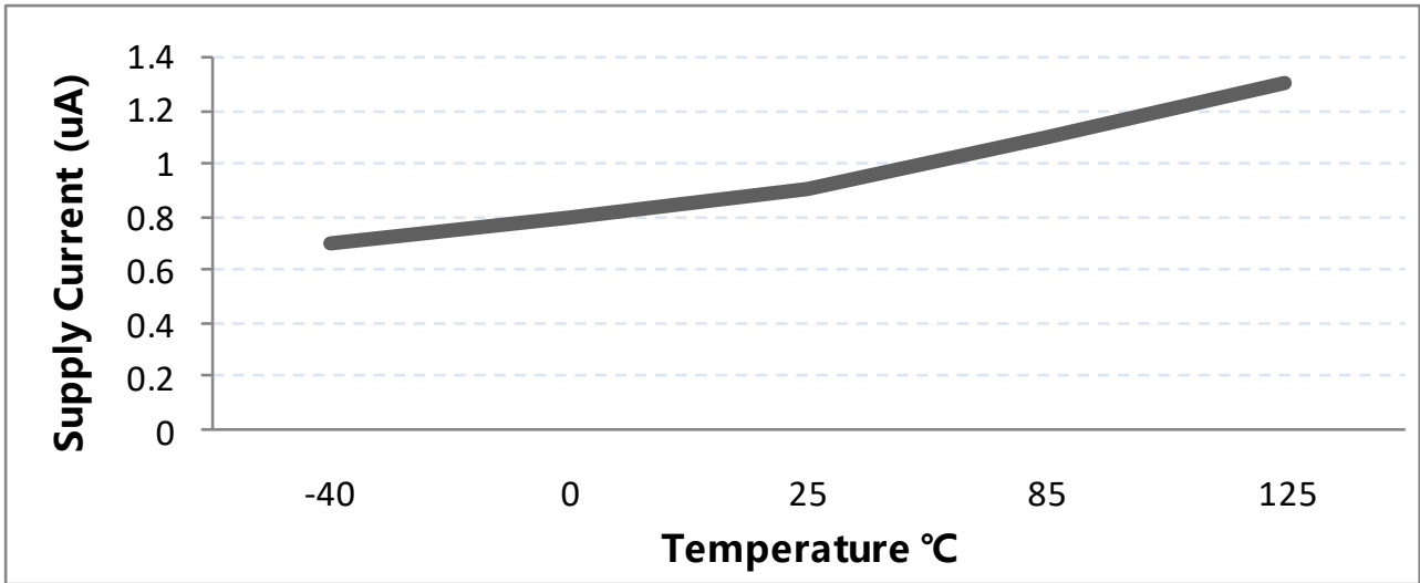
Figure.5 Average Supply Current vs. Temperature
